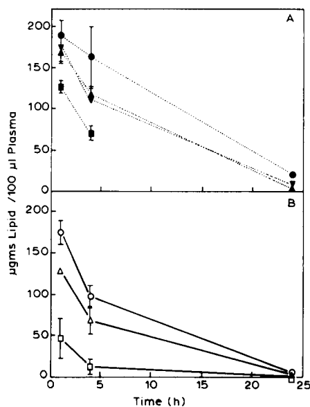
Fig. 7. In vivo clearance rates of protein-liposome conjugates. Streptavidin was coupled to liposomes (50 and 100 nm), at a final lipid concentration of 30 mM and incubation period of 15 min, quenched with N -ethylmaleimide for 2 h followed by an overnight incubation with \beta -mercaptoethanol. Control liposomes containing MPB-DPPE were titrated to pH 7.5 and exchanged on Sephadex G-50 equilibrated with HBS. EPC/cholesterol liposomes were made up in HBS. Mice (4–8 mice per time point) were injected with lipid at a dose of 100 mg/kg. Plasma was prepared from EDTA treated whole blood at specific time points and aliquots were analyzed by scintillation counting (see Materials and Methods for details). Size of extruded samples were determined by QELS. (A) EPC/cholesterol, 125 nm (●); EPC/cholesterol, 197 nm (■); MPB-DPPE liposomes, 170 nm (quenched ▲, unquenched ▼). (B) Aggregated 100 nm streptavidin-liposomes, 530 nm (□); streptavidin-liposomes extruded through 100 nm, 187 nm (Δ); streptavidin-liposomes extruded through 50 nm, 139 nm (○).
