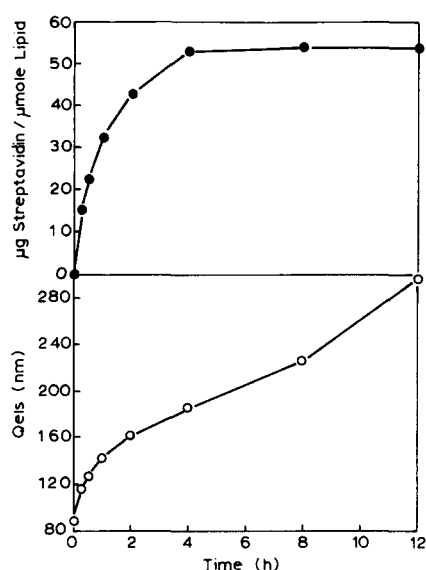
Fig. 1. Effect of coupling streptavidin to liposomes on vesicle size. Liposomes (54 mol% EPC, 45 mol% CHOL, 1 mol% MPB-DPPE, 5 mM final lipid concentration, 100 nm) were incubated with streptavidin (100 µg protein/µmol lipid) over time at pH 7.5. At various time points, the reaction was quenched by addition of N -ethylmaleimide (500 molar ratio to protein) and free streptavidin was removed by gel filtration on Sepharose CL-4B. Extent of coupled streptavidin was determined by [ 3 H]biotin binding (top figure) and vesicle size was estimated by QELS (bottom figure).
