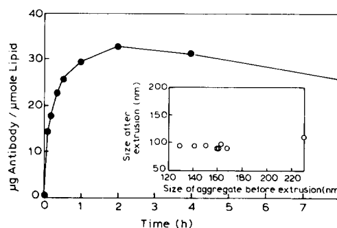
Fig. 4. Extrusion of antibody-liposome conjugates. Fluorescein-labelled antibody was coupled to liposomes (100 nm) containing 1% MPB-DPPE at a final lipid concentration of 20 mM. At various time points aliquots of the reaction mixtures were quenched with N -ethylmaleimide and diluted to 5 mM lipid concentration before extrusion through 100 nm filters. The extent of coupled antibody (●) was determined by estimating the levels of liposomally associated fluorescence after extrusion and exchange of lipid samples on Sepharose CL-4B. The size of the antibody-liposome conjugates was estimated by QELS before and after (inset, ○) extrusion as described in Materials and Methods.
