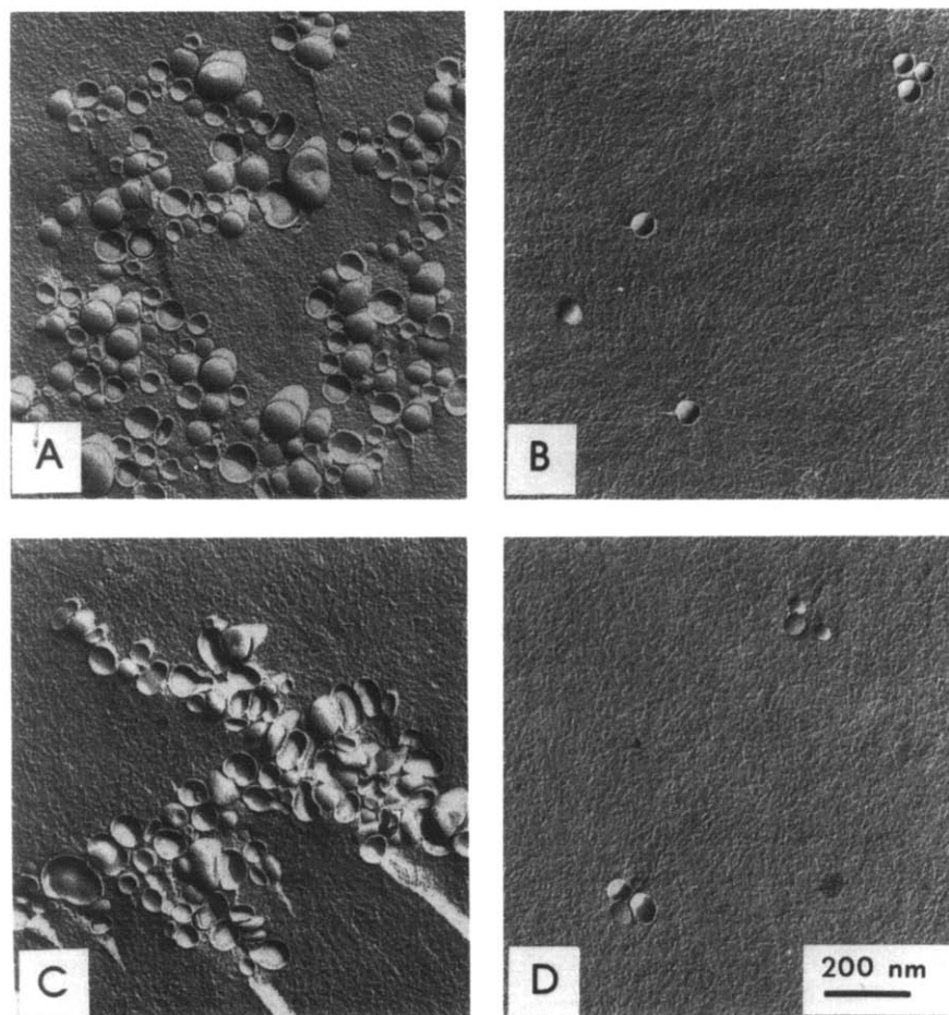
Fig. 5. Freeze-fracture of streptavidin-liposomes before and after extrusion. Streptavidin was coupled to liposomes at a final lipid concentration of 20 mM for 8 h as described in Fig. 1. The sample was diluted to 5 \mu mol/ml prior to extrusion. Non-covalent attachment of streptavidin to liposomes containing biotin EPE (0.25 mol%) was performed as described in Materials and Methods at a final lipid concentration of 5 mM. Samples were examined by freeze-fracture before and after extrusion through 100 nm filters. Streptavidin-liposomes containing MPB-DPPE before (A) and after (B) extrusion; streptavidin-liposomes containing biotin EPE before (C) and after (D) extrusion.
