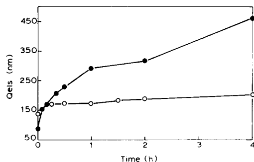
Fig. 6. Examination of the stability of extruded streptavidin-liposome conjugate by QELS. Streptavidin-liposomes with approx. 51 \mu g protein/ \mu mole lipid were prepared by incubating thiolated streptavidin with liposomes containing 1 mol% MPB-DPPE for 8 h at a final lipid concentration of 20 mM. After removal of unbound streptavidin by gel filtration on Sepharose CL-4B, the sample was diluted to 5 mM lipid and extruded 10 times through two stacked 100 nm filters. At various time points the size of the extruded preparation was determined by QELS (○). Size of streptavidin-liposome conjugates prepared as in Fig. 1 are shown for comparison (●).
