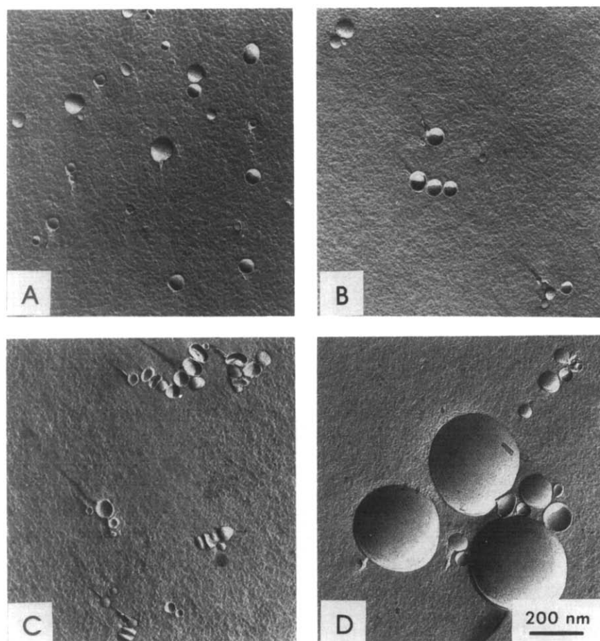
Fig. 2. Freeze-fracture of streptavidin-liposome preparations. Streptavidin-liposome samples quenched with N -ethylmaleimide at 0.5 (A), 2 (B), 4 (C) and 18 (D) h were prepared as described in Fig. 1 and examined by freeze-fracture.
