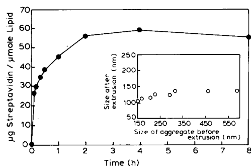
Fig. 3. Extrusion of streptavidin-liposome conjugates. Streptavidin was coupled to liposomes (100 nm) containing 1 mol% MPB-DPPE at a final lipid concentration of 20 mM. At various time points aliquots of the reaction mixtures were quenched with N -ethylmaleimide and diluted to 5 mM lipid concentration before extrusion through 100 nm filters. The extent of coupled streptavidin (●) was estimated by [ ^3 H]biotin binding to streptavidin-liposomes after extrusion and gel exclusion of lipid samples on Sepharose CL-4B. The size of the liposome streptavidin conjugates was estimated by QELS before and after (inset, ○) extrusion as described in Materials and Methods.
